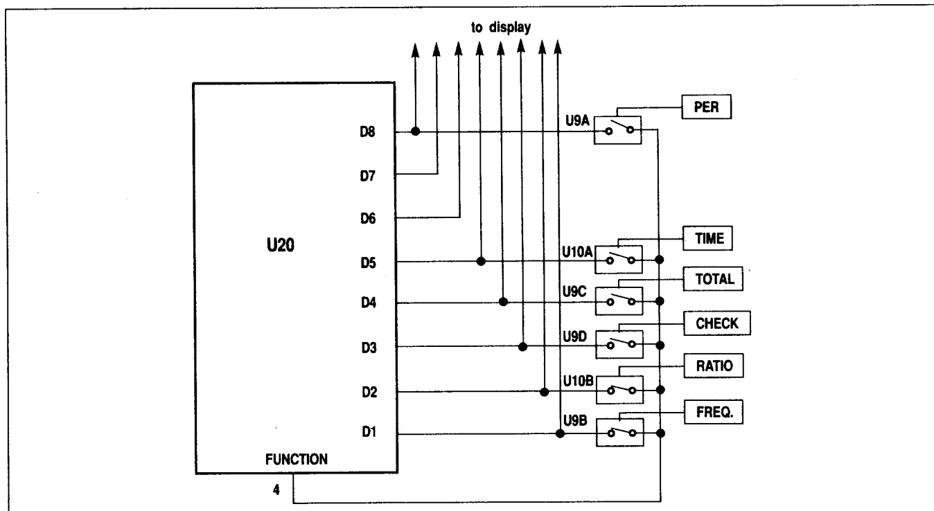
Figure 7. Function Selection.
