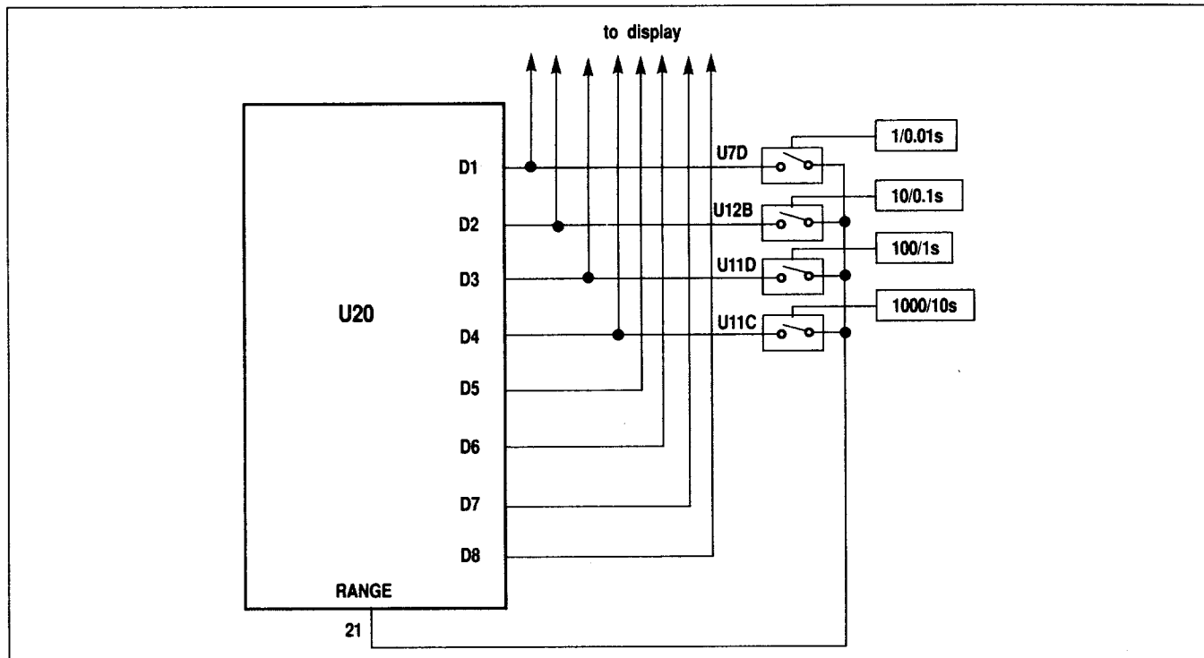
Figure 8. Gate Selection.
