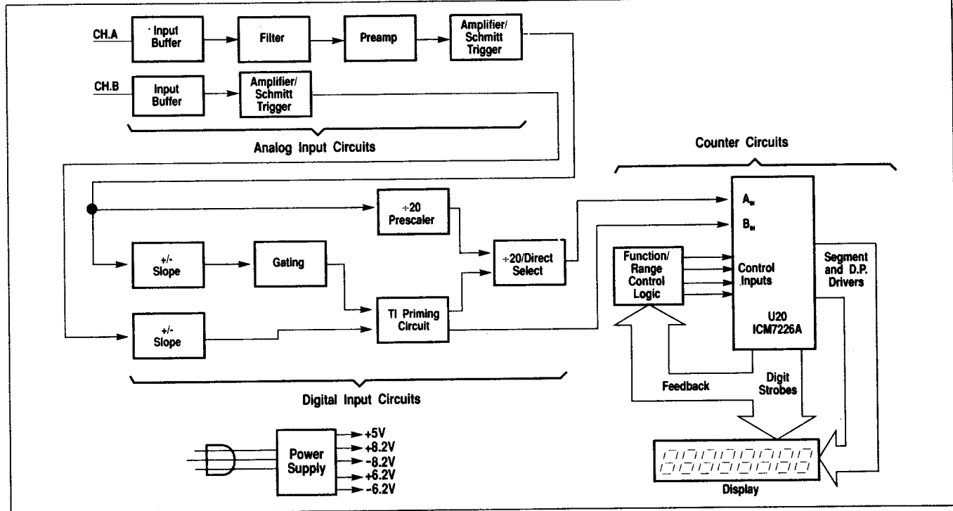
Figure 5. Block Diagram.
