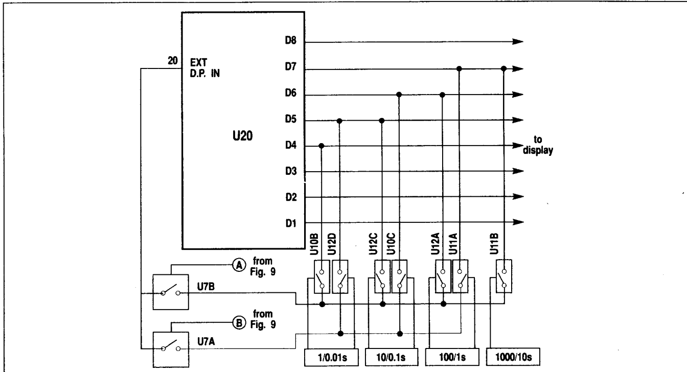
Figure 11. External Decimal Point Control.
