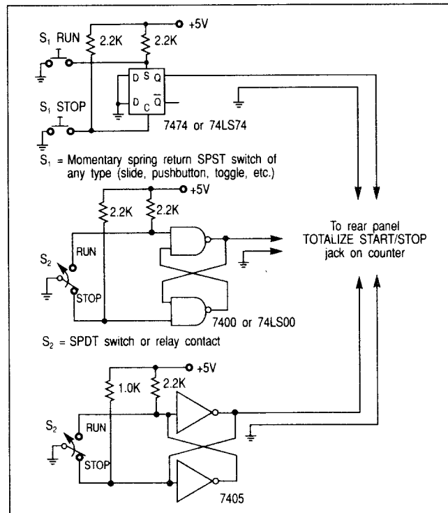
Figure 15. Debouncing Circuits.
